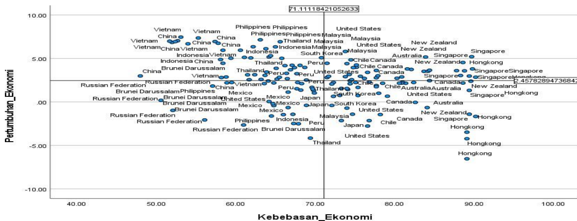
Figure 2. Quadrant Diagram
